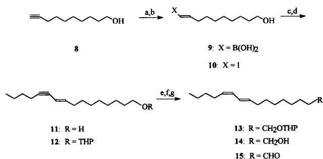
Scheme 2. (a) i. Catecholborane, ii. H 2 O; (b) i. NaOH, H 2 O, ii. I 2 ; (c) Hexyne, (Ph 3 P) 2 PdCl 2 , CuI, diisopropylamine; (d) DHP, H + ; (e) i. Dicyclohexylborane, ii. AcOH; (f) MeOH, H + ; (g) Swern oxidation.
